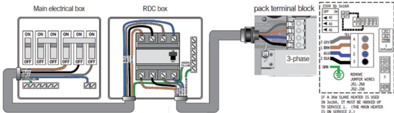
Electrical wiring: European model
