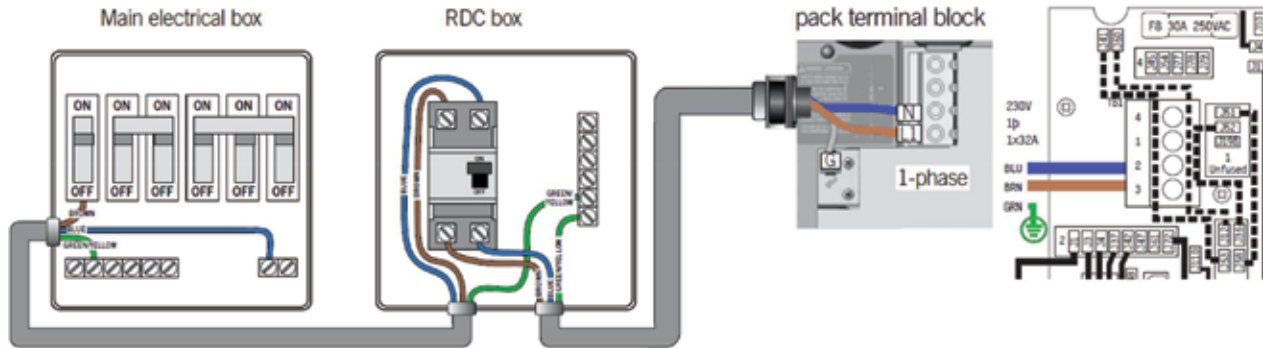
Electrical wiring: European model
